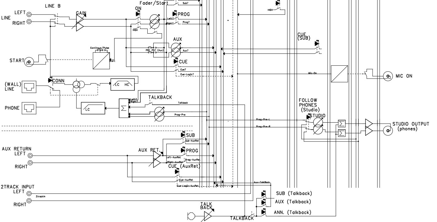
AIRMATE-USB SIGNAL FLOW
